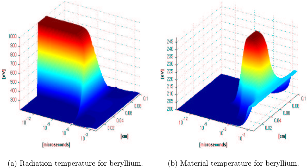
Fig. 3. Radiation and material temperatures for 1D radiation diffusion through beryllium shown as surface plots across time and space for the closed system model problem.
