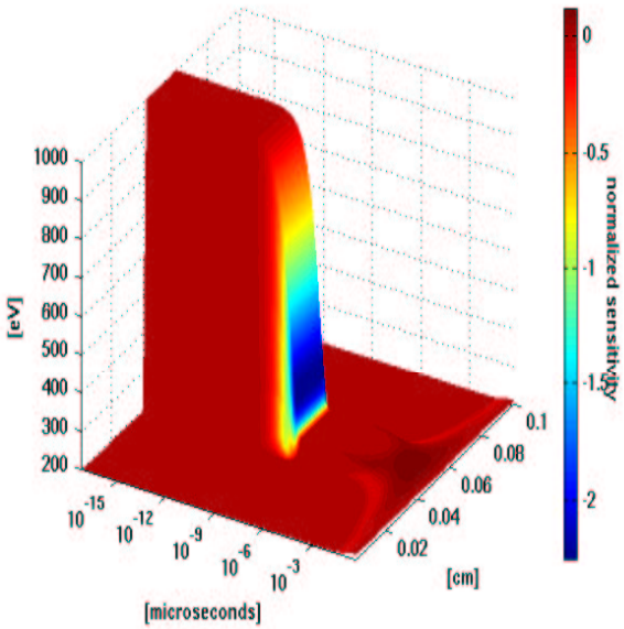
(a) Radiation temperature.
