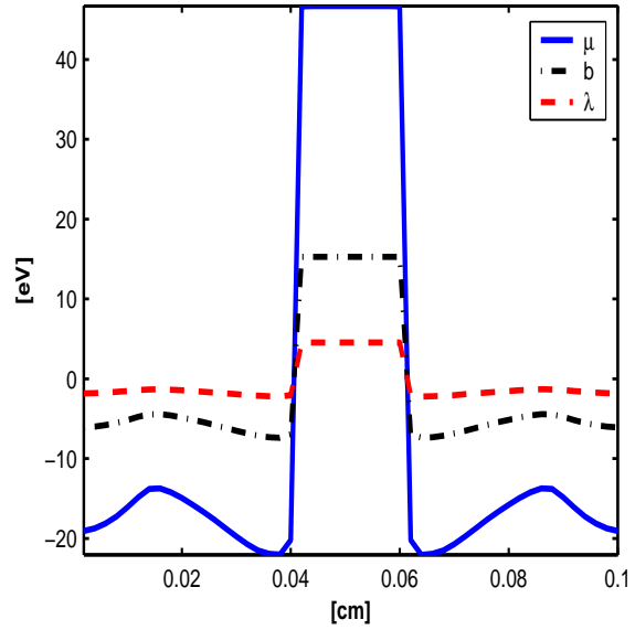
(b) Maximum scaled sensitivity for T_M .
