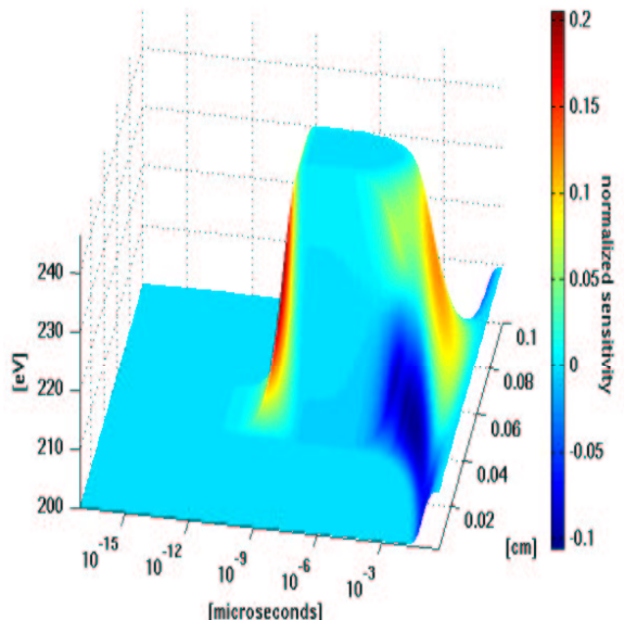
(b) Material temperature.
