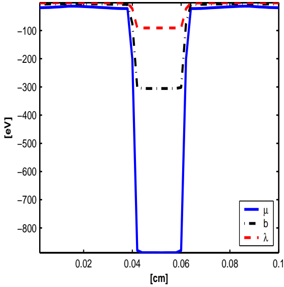
(a) Maximum scaled sensitivity for T_R .
