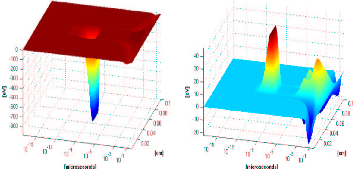
(a) Scaled sensitivity for radiation temperature in aluminum.
