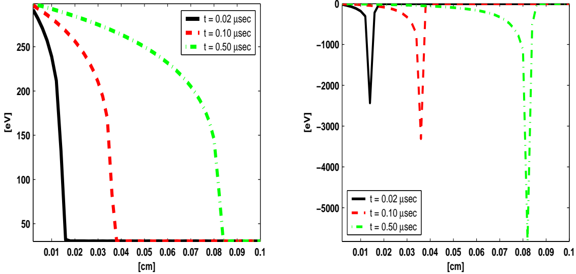
(a) Radiation temperature for aluminum.
