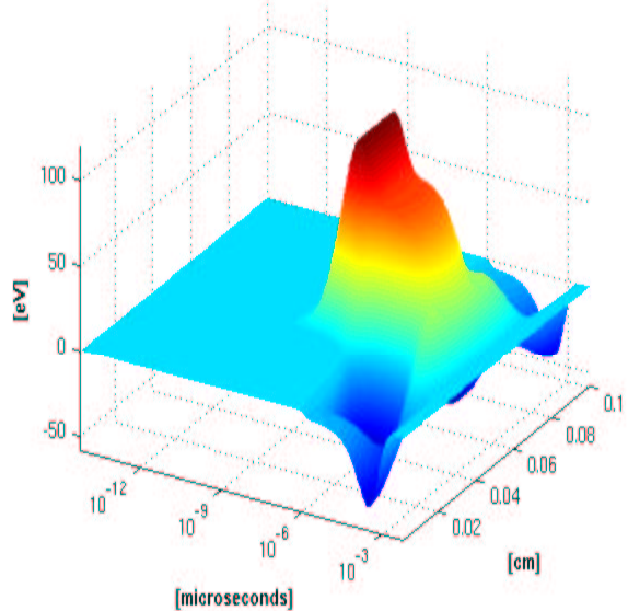
(b) Scaled sensitivity for material temperature in beryllium.
