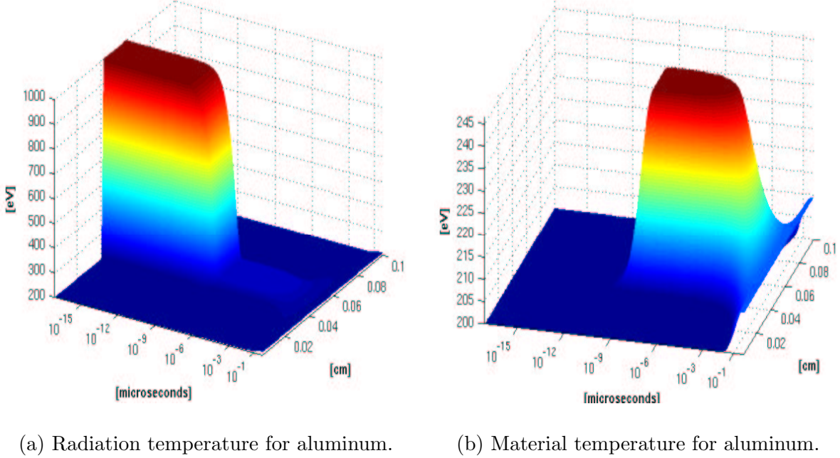
Fig. 1. Radiation and material temperatures for 1D radiation diffusion through aluminum shown as surface plots across time and space for the closed system model problem.
