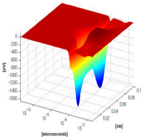
(a) Scaled sensitivity for radiation temperature in beryllium.
