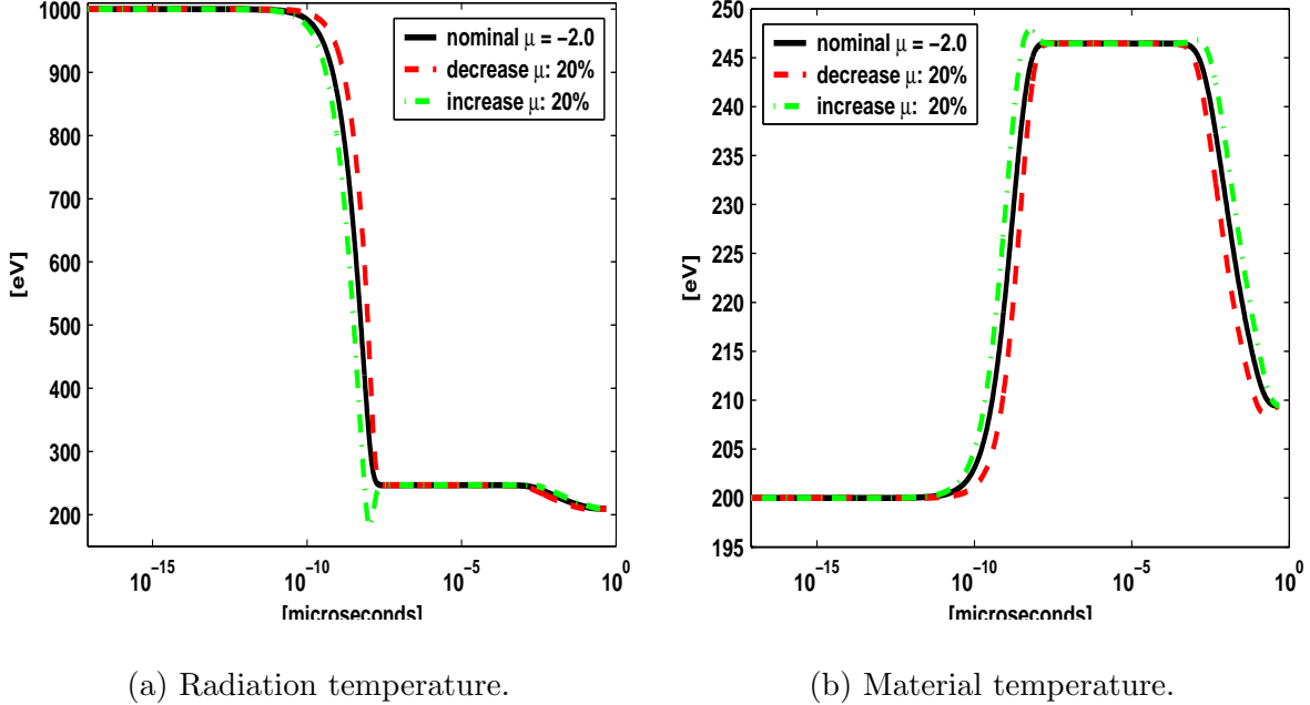
Fig. 8. Radiation and material temperatures, with error bars associated with \pm 20\% uncertainty in the temperature exponent for radiation diffusion through aluminum in the closed system.
