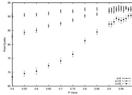
Fig. 6. Mean real quality for different noise levels varying the parameter p .
