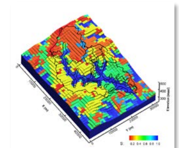
Subsurface flow
