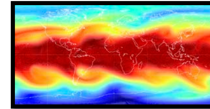
Atmospheric Dynamics
